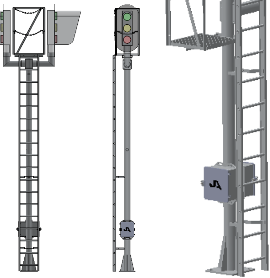
REF C—Top Platform Only
